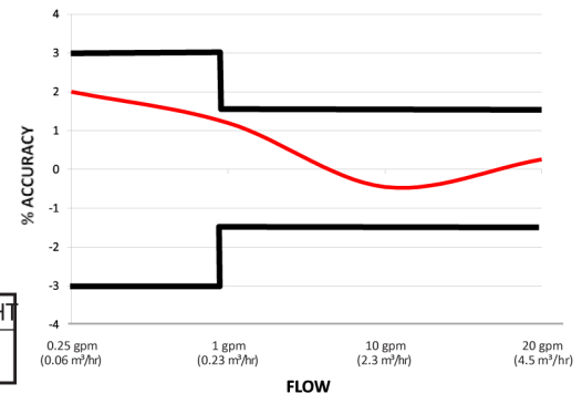
Accuracy Chart
